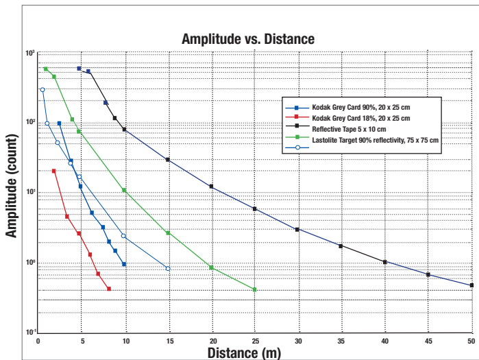
The chart below displays the detection amplitude of a 45° sensor for five reference objects (photography grey cards and reflective tape) of varying size and reflectivity.
