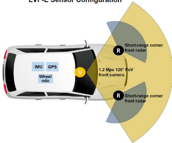
LVE-E Sensor Configuration
