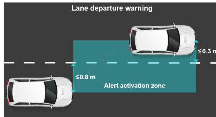
Figure 4 – Existing lane departure warning alert activation criteria
